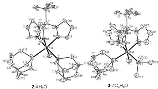
Figure 3. Molecular structure and atom labeling scheme for 2 ·4H 2 O and 3 ·2C 3 H 6 O. Solvent molecules and hydrogen atoms have been omitted for clarity. Non-hydrogen atoms are represented by 50% probability ellipsoids.
