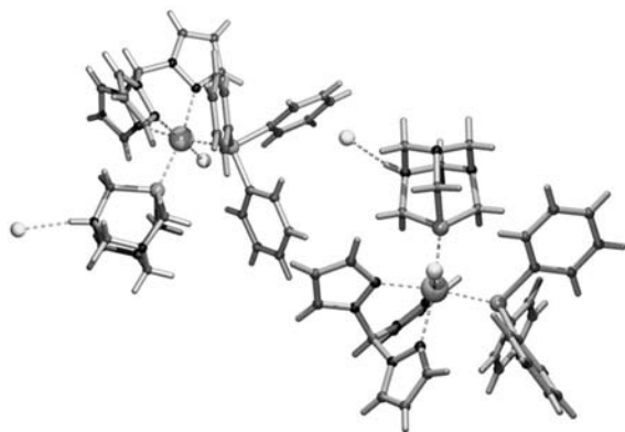
Figure 5. Hydrogen bonding in 6b .
