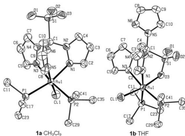
Figure 2. Molecular structure and atom labeling scheme for 1a · \text{CH}_2\text{Cl}_2 and 1b ·THF. Solvent molecules and hydrogen atoms have been omitted for clarity. Non-hydrogen atoms are represented by 50% probability ellipsoids.
