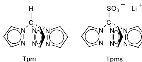
Figure 1. Tpm and Tpms ligands.
