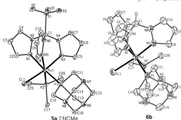
Figure 4. Molecular structure and atom labeling scheme for the complex cations of 5a ·2NCMe and 6b . Solvent molecules and hydrogen atoms, except N–H, and the apical hydrogen atom of Tpm are omitted for clarity. Non-hydrogen atoms are represented by 50% probability ellipsoids.
